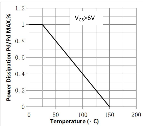
Fig.3 Power Dissipation
